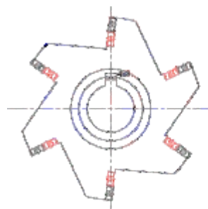
Special Slot Milling Cutter
