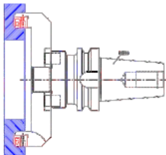
Special Trepaning cum Grooving Tool
