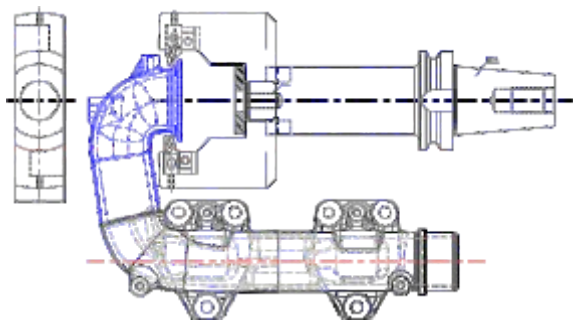
Special O.D. Turning cum Chamfer Tool
