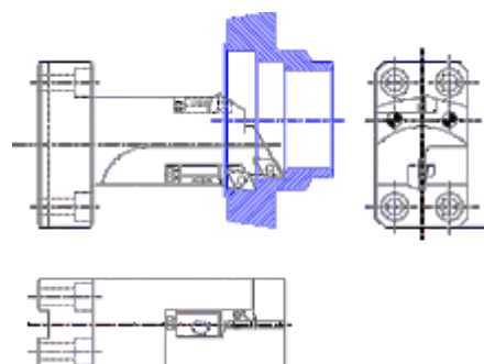
Special Finish cum Chamfer Tool
